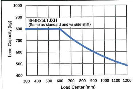
Load capacity charts
