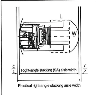
Right-angle stacking (SA) aisle width
