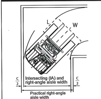
Intersecting (IA) and right-angle aisle width
